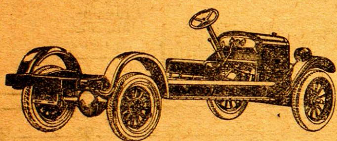
CHASSIS CAMION
